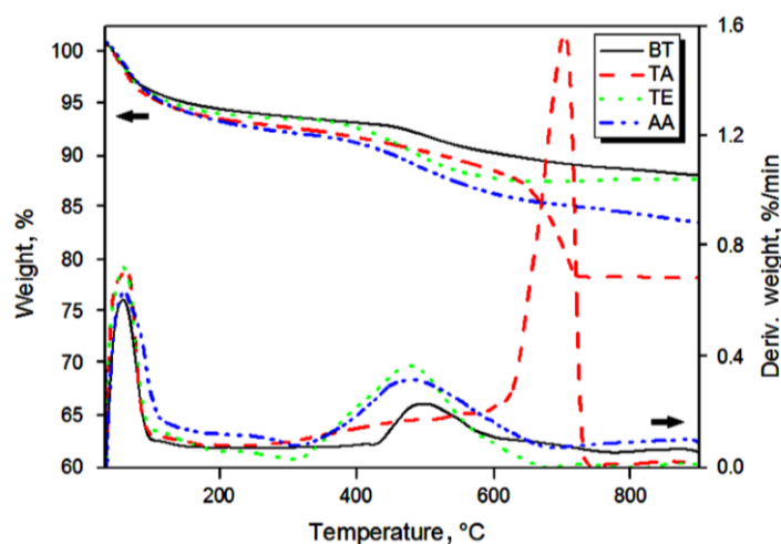
Fig. 3. TG and DTG curves of bituminous rock samples.
