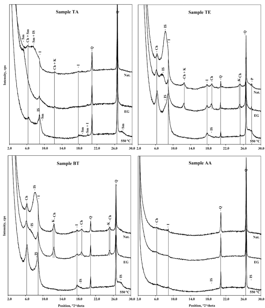
Fig. 5. X-ray diffraction analyses of the < 2 μm fraction of the four studied samples: Nat – untreated sample; EG – glycolated sample; H – sample heated to 550 °C; Ch – chlorite; IS – interstratified illite and smectite; I – illite; K – kaolinite; Q – quartz; P – plagioclase.
