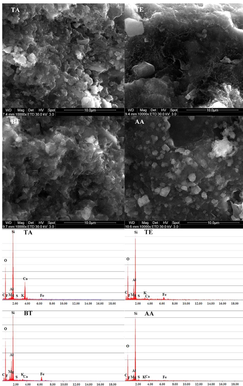
Fig. 6. SEMs for the bituminous rock samples studied.
