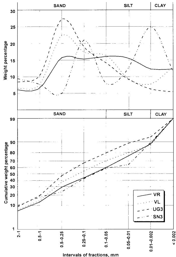
Fig. 2. Distribution and cumulative curves of the average composition of different till units. VR, Vörtsjärve; VL, Valgjärve; UG3, Upper Ugandi; SN3, Upper Sangaste.
